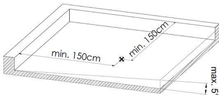
Attika
